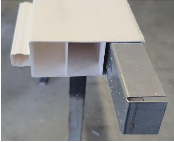
Aluminium reinforced profile
