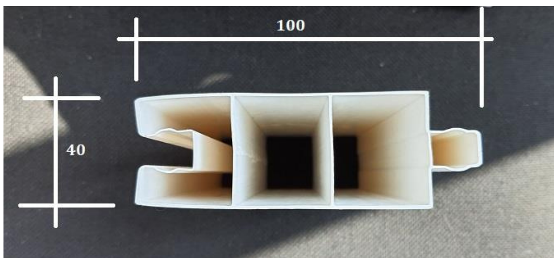
Profile used for the roof
